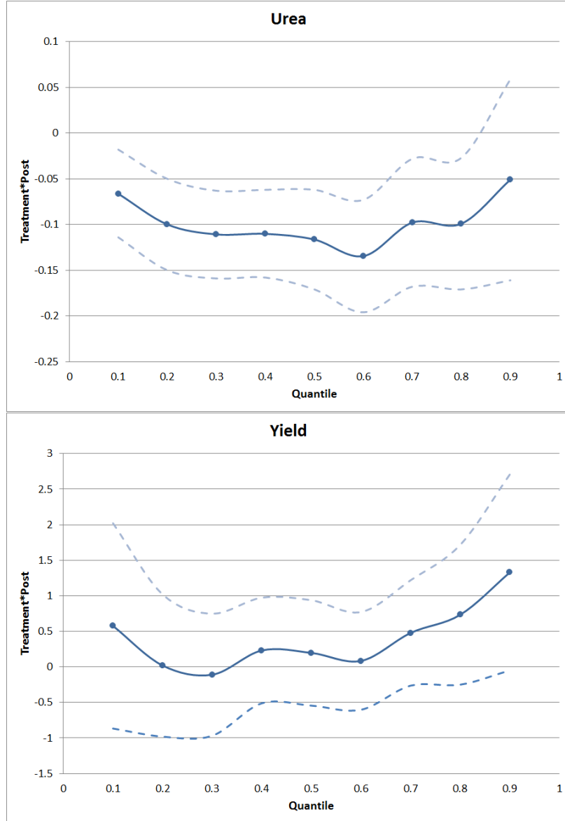
Figure 2: Quantile Regressions
